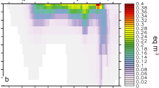
DIC concentration difference (year 2099 minus year 2020)
