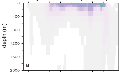
DIC concentration difference (year 2059 minus year 2020)
