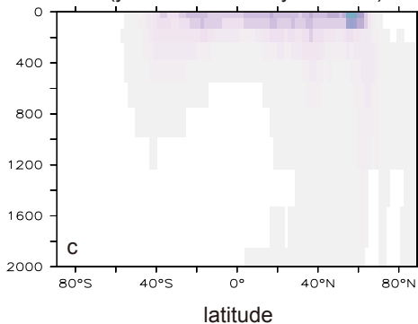
DIC concentration difference (year 2059 minus year 2020)
