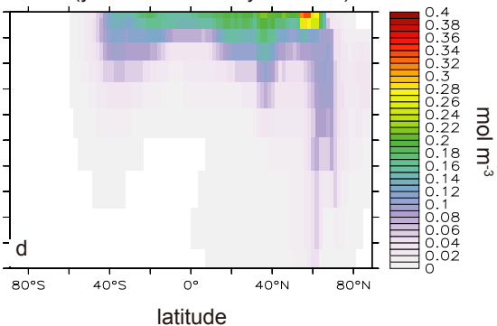
DIC concentration difference (year 2099 minus year 2020)
