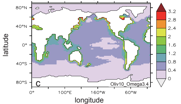
sea surface aragonite Ω difference
