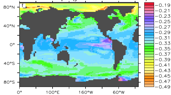
sea surface pH (year 2099 minus 2020)
