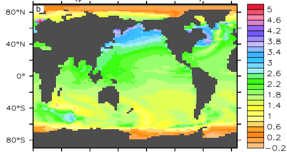
sea surface aragonite \Omega (year 2099 minus 2020)
