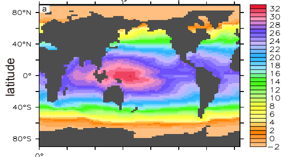
sea surface aragonite \Omega (year 2020)
