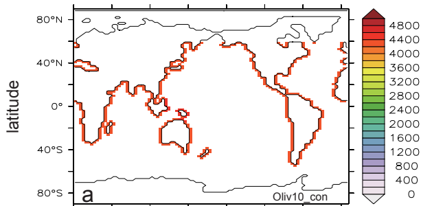
sea surface aragonite Ω difference
