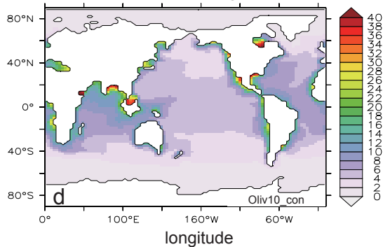
sea surface aragonite Ω
