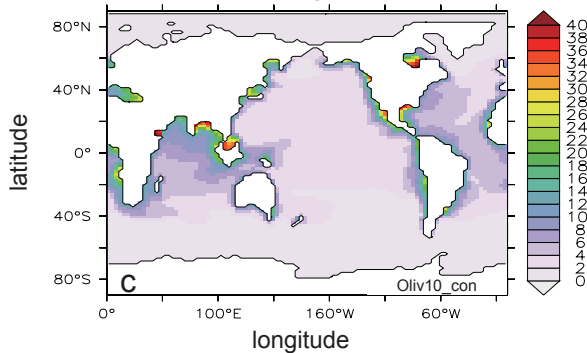
sea surface aragonite Ω difference
