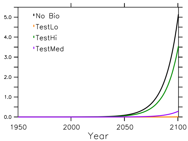
a Total Surface MP (particles m^{-3} )
